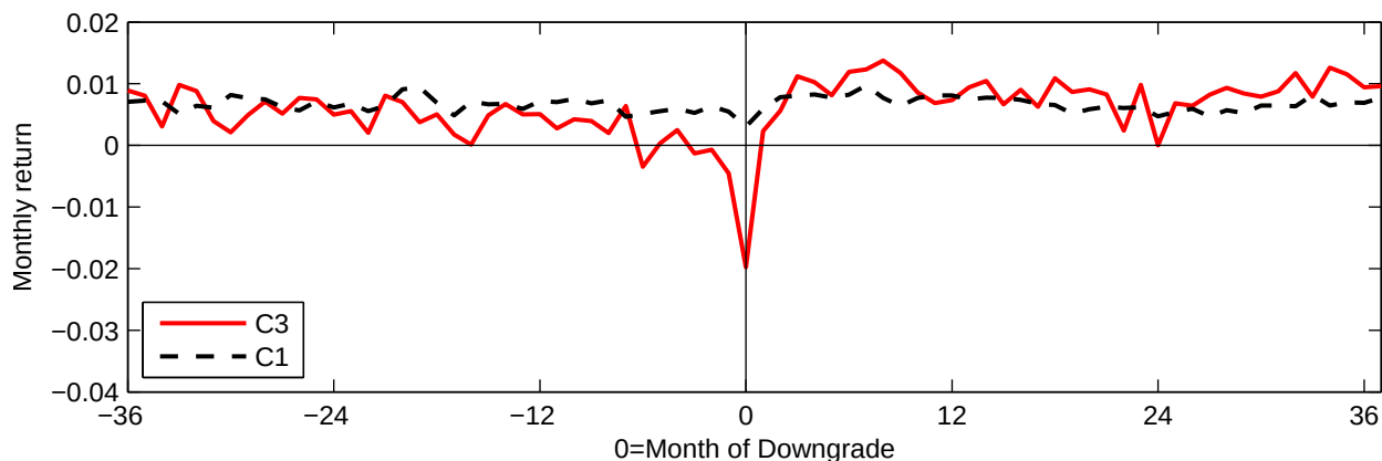
Plot B: Impact of downgrades on bond returns in high sentiment (Annual \text{SENT}_{t-1}^\perp > 0 )
