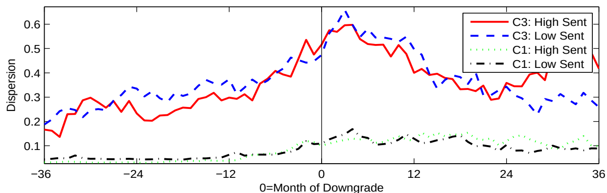
Figure 3. Impact of downgrades on fundamental uncertainty in high and low sentiment. We repeat the sorts in Figure 2, but examine the change in fundamental uncertainty around downgrades following high or low monthly sentiment.
