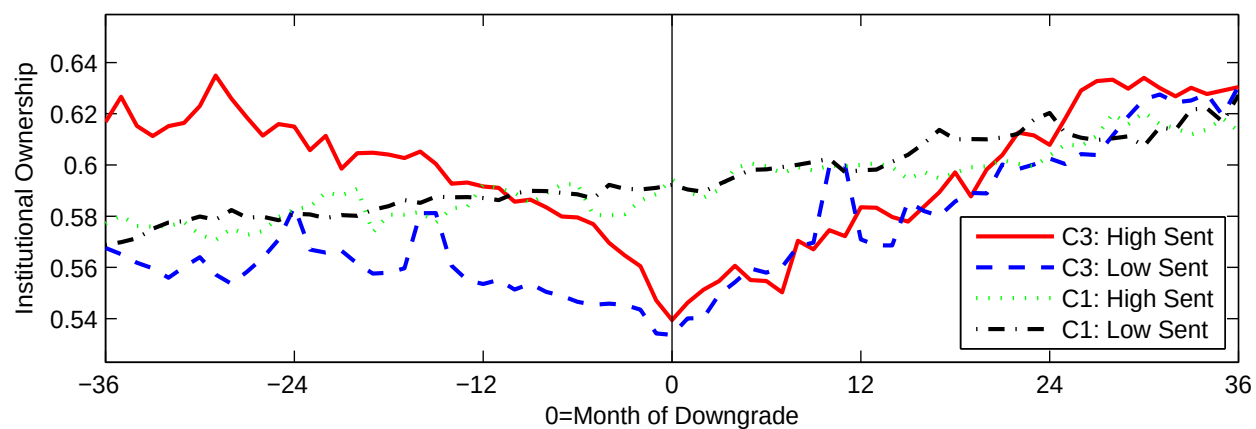
Figure 4. Institutional ownership around downgrades following high and low sentiment. We repeat the sorts in Figure 2, but examine institutional ownership following high or low monthly sentiment. Institutional ownership is measured as the number of shares held by institutions (from Thompson Financial) as a percentage of total shares outstanding.
