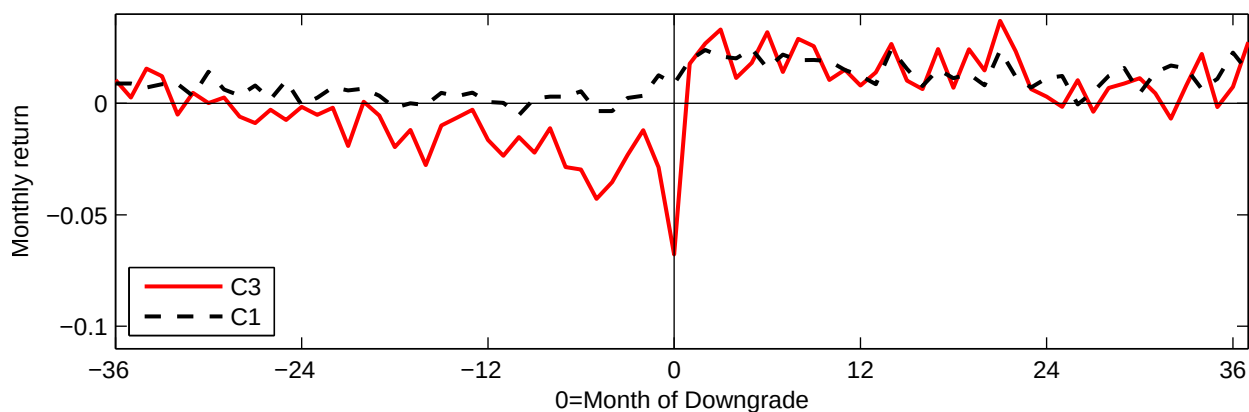
Plot D: Impact of downgrades on stock returns in high sentiment (Annual \text{SENT}_{t-1}^\perp > 0 )
