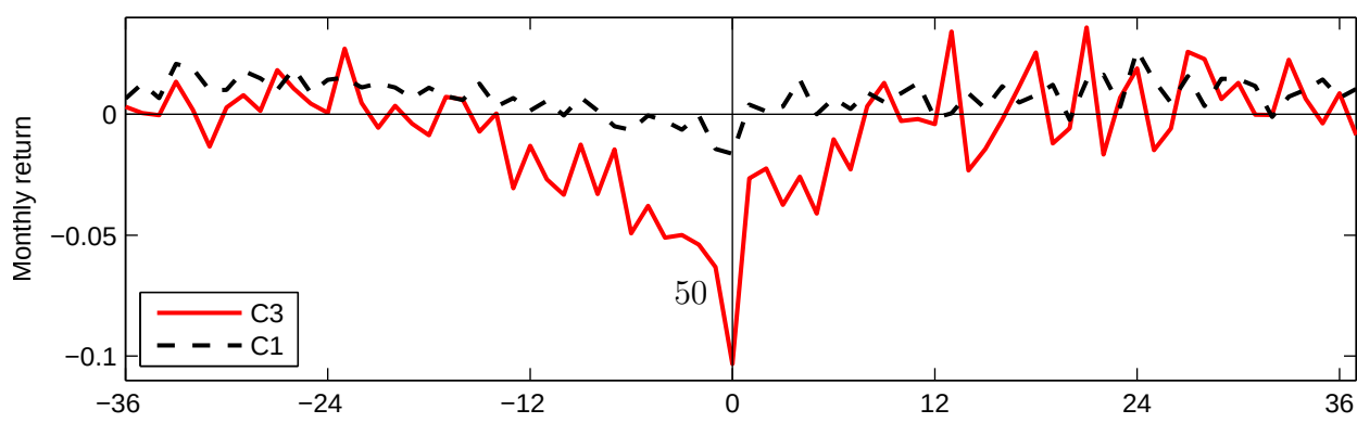
Plot D: Impact of downgrades on stock returns in high sentiment (Annual \text{SENT}_{t-1}^\perp > 0 )
