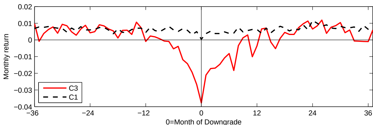
Plot C: Impact of downgrades on stock returns in low sentiment (Annual \text{SENT}_{t-1}^\perp < 0 )
