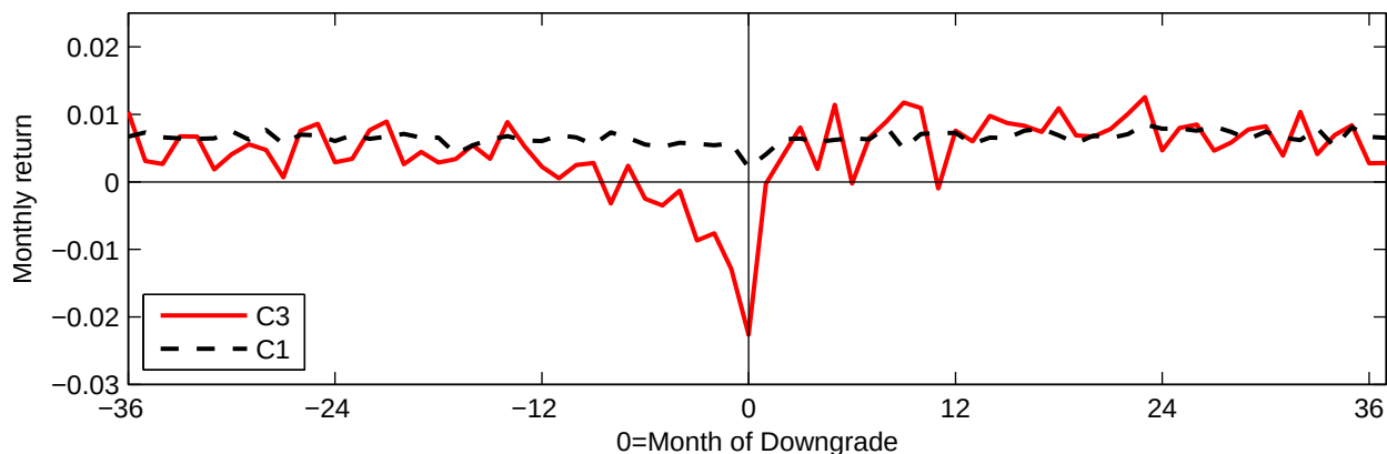
Plot B: Impact of issuer downgrades on bond returns of underpriced firms
